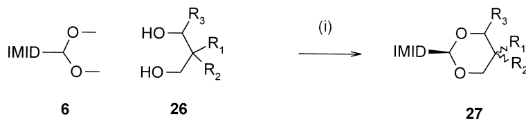
Scheme 3. General method A, library 1 (see Table 1 for the list of diols 26 ). (i) General method A: 4-toluenesulphonic acid, CH 2 Cl 2 .
