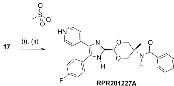
Scheme 10. Preparation of RPR201227A. (i) Benzoic acid, HATU, DIPEA, DMF; (ii) CH 3 SO 3 H, THF, rt.
